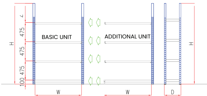
DETAIL FRONT & SIDE VIEW OF RACK SCALE 1 : 30
