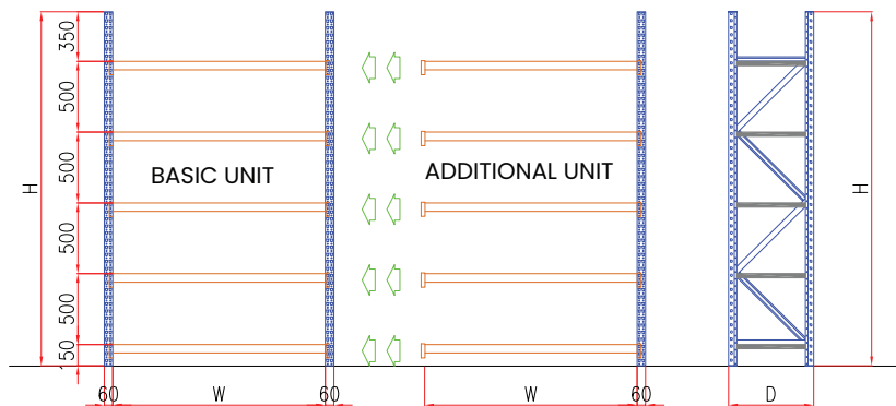
DETAIL FRONT & SIDE VIEW OF RACK SCALE 1 : 30
